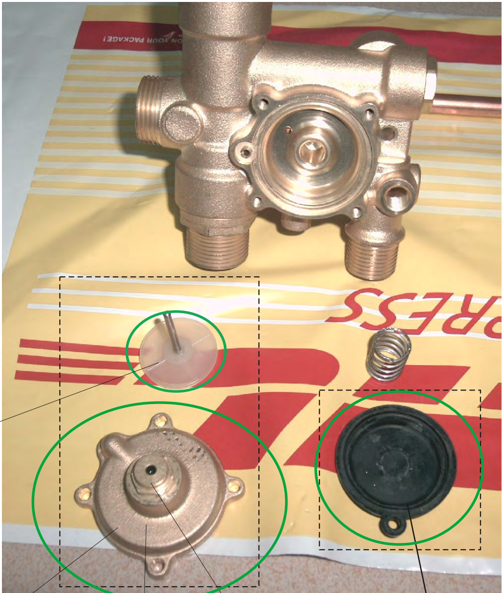
Piston of the water pressure switch Code:70102004
